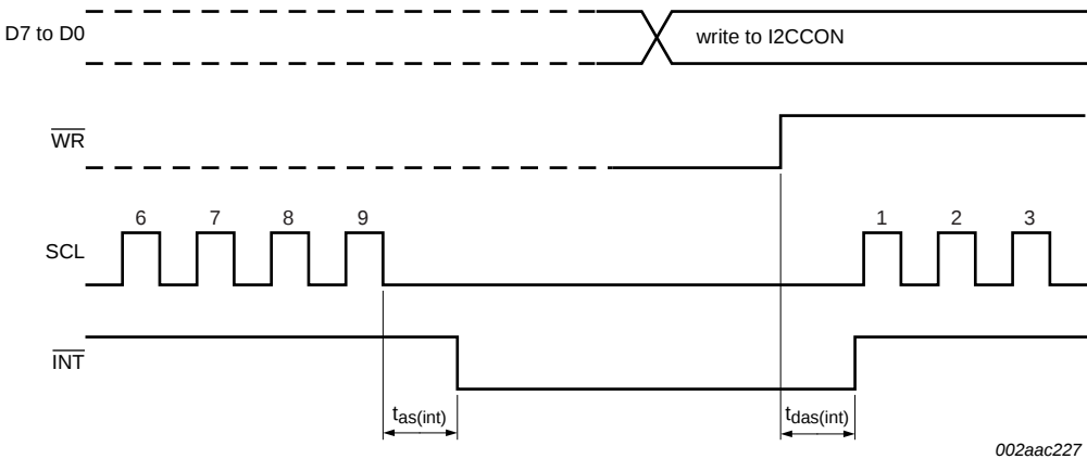
Fig 40. Interrupt timing
