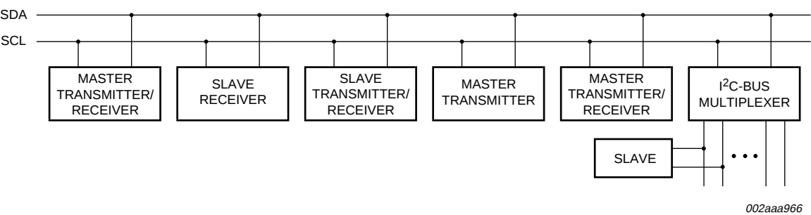
Fig 30. System configuration
