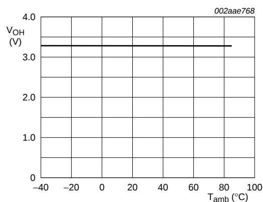
Fig 19. V_{OH} at V_{DD} = 3.3 \text{ V} , V_{DD(I/O)n} = 3.3 \text{ V} , I_{OH} = -1 \text{ mA}
