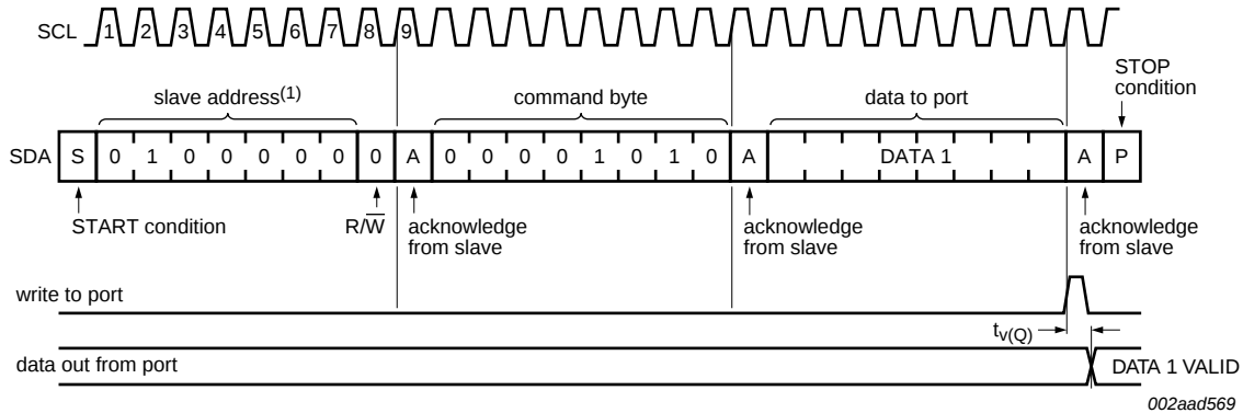
Fig 13. Write to Output port register
