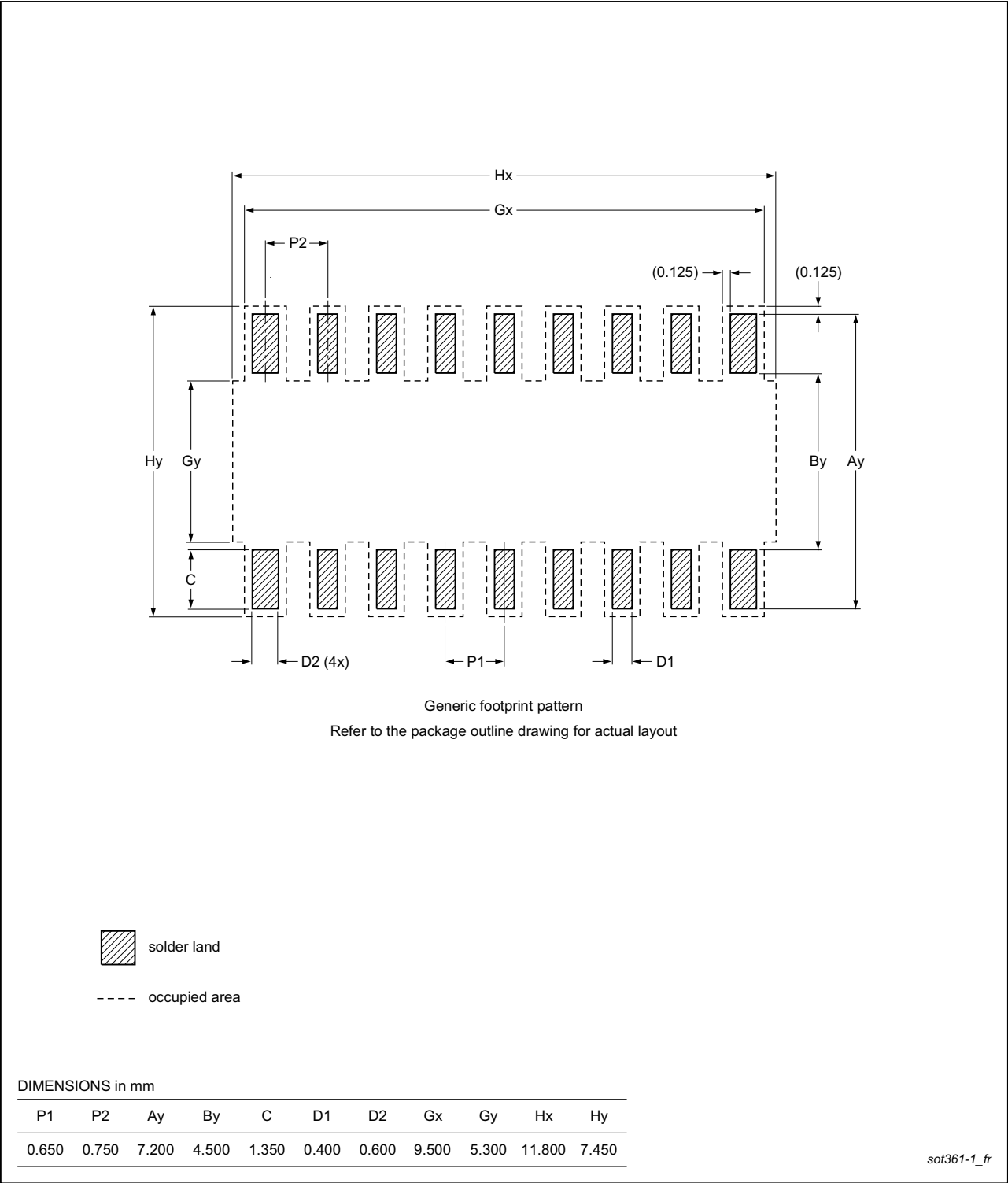
Fig 30. PCB footprint for SOT361-1 (TSSOP28); reflow soldering
