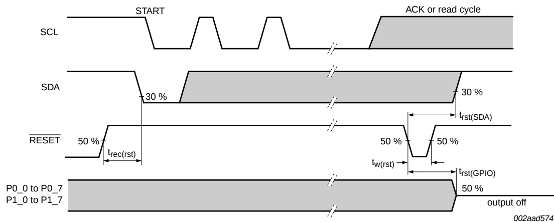
Fig 23. Reset timing
