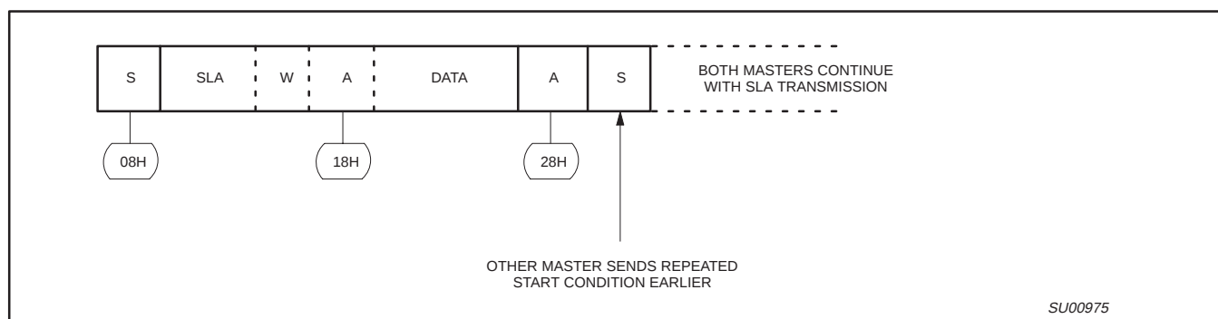
Figure 6. Simultaneous repeated START conditions from 2 masters
