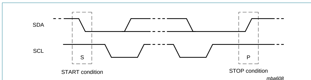
Fig 11. Definition of START and STOP conditions
