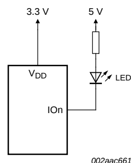
Fig 20. Device supplied by a lower voltage
