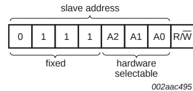
Fig 10. PCA9554A device address
