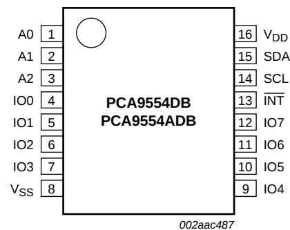
Fig 3. Pin configuration for SSOP16
