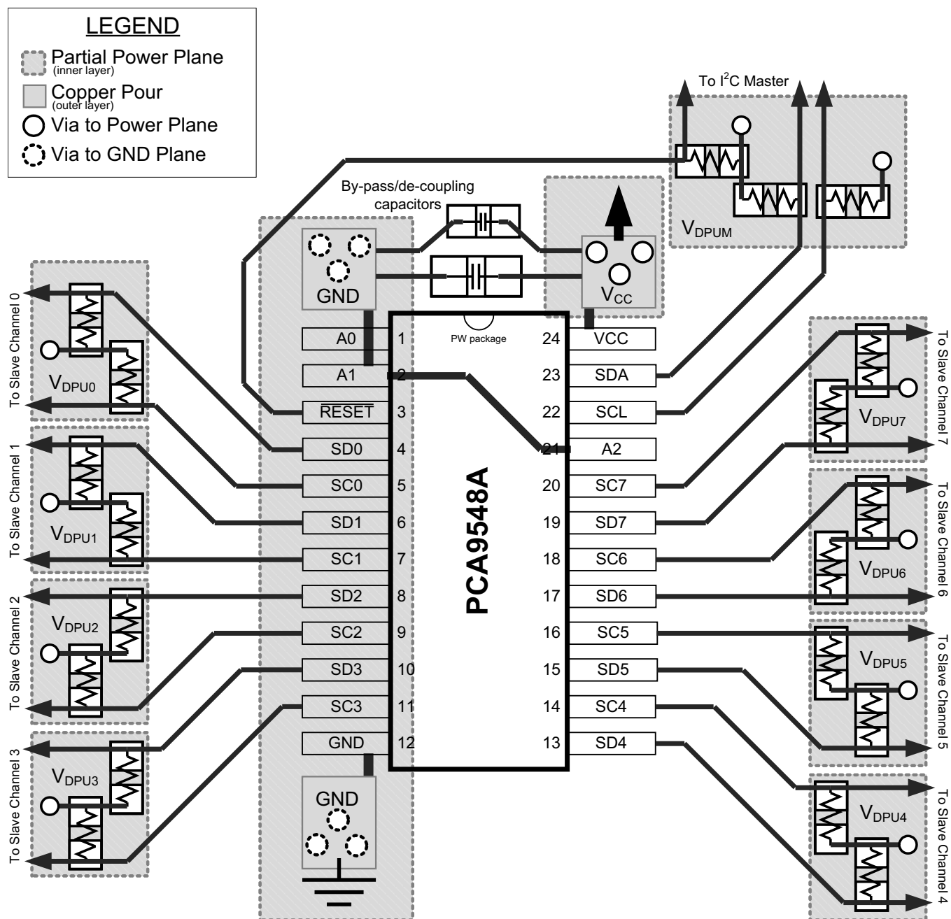
Figure 17. Layout Example
