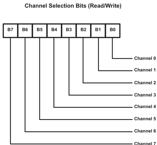
Figure 9. Control Register
