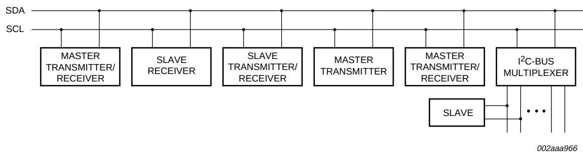
Fig 10. System configuration
