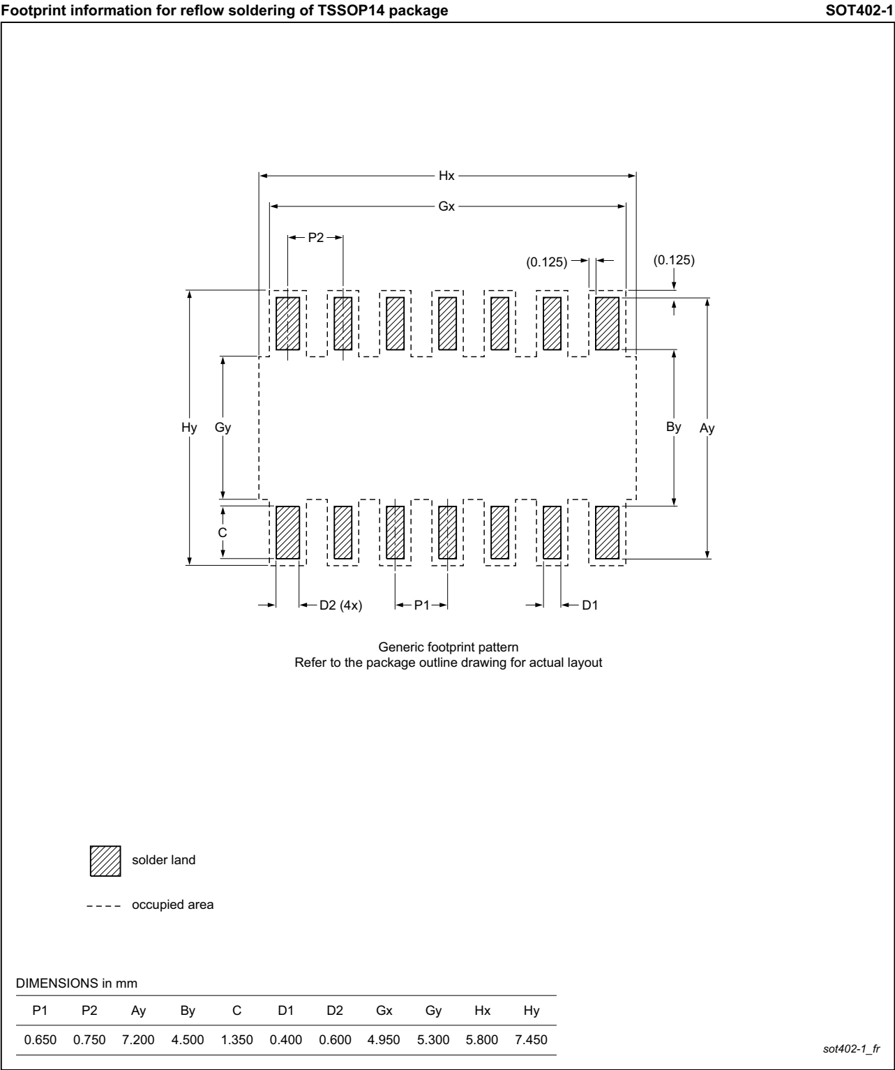
Fig 22. PCB footprint for SOT402-1 (TSSOP14); reflow soldering
