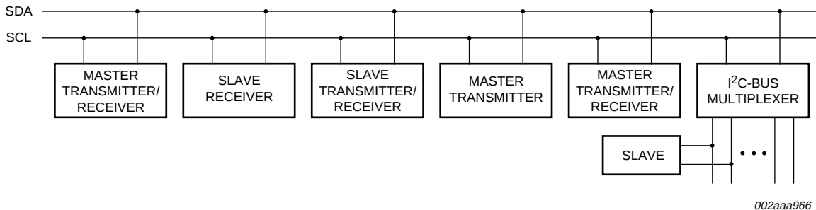
Fig 17. System configuration
