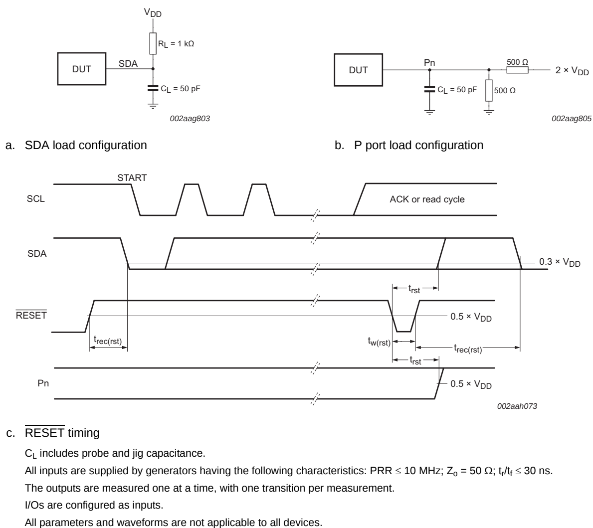
Fig 29. Reset load circuits and voltage waveforms
