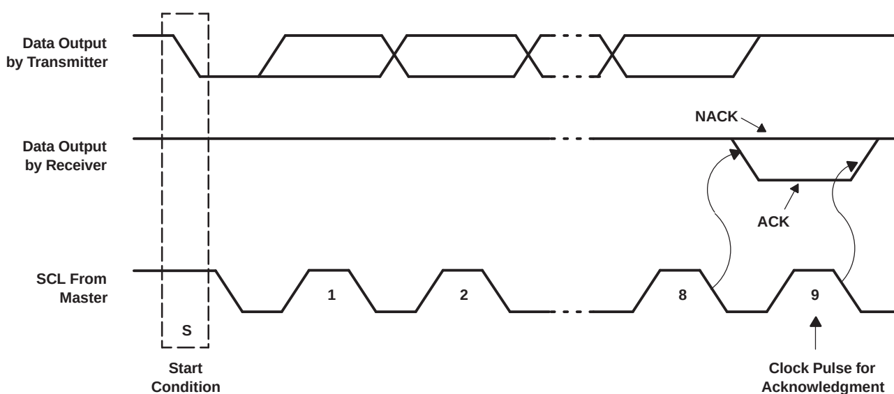
Figure 20. Acknowledgment on the I²C Bus
