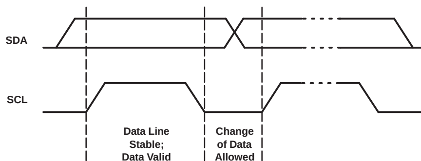
Figure 19. Bit Transfer
