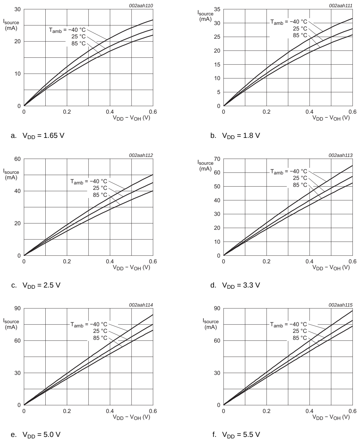
Fig 23. I/O source current versus HIGH-level output voltage
