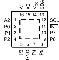
RGT PACKAGE (TOP VIEW)
