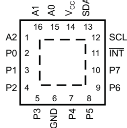
RGV PACKAGE (TOP VIEW)
