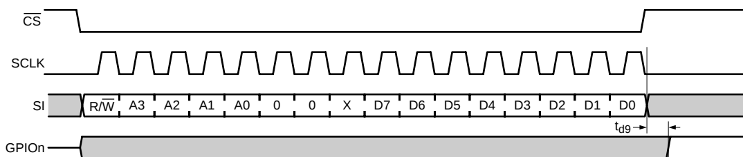
Fig 17. SPI write IOState to GPIO switch
