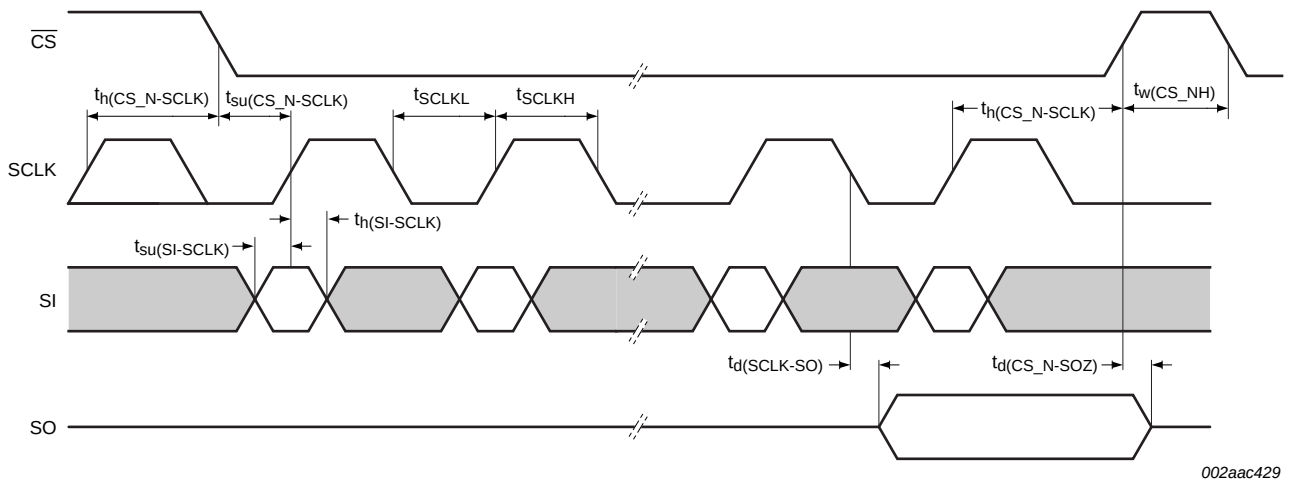
Fig 16. Detailed SPI-bus timing
