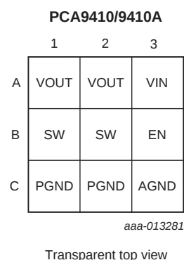
Fig 3. Ball mapping for WLCSP9
