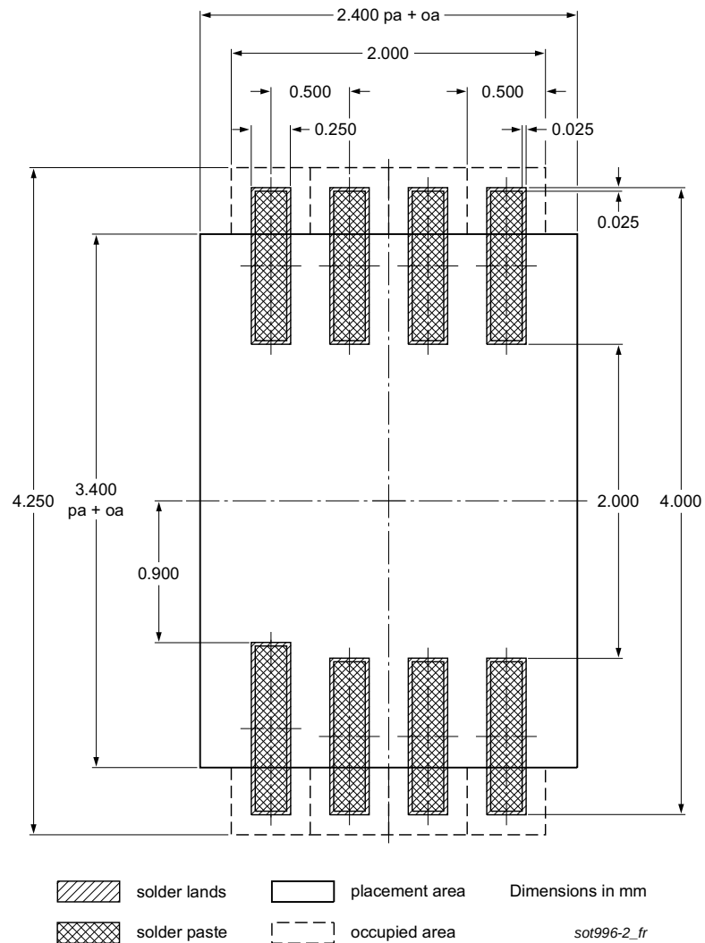
Fig 28. PCB footprint for SOT996-2 (XSON8U); reflow soldering
