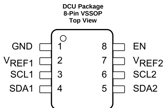
Pin Functions
