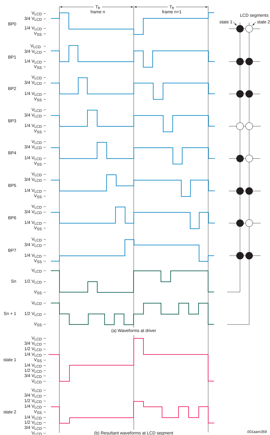
Fig 19. Waveforms for 1:8 multiplex drive mode with bias \frac{1}{4} and frame inversion
