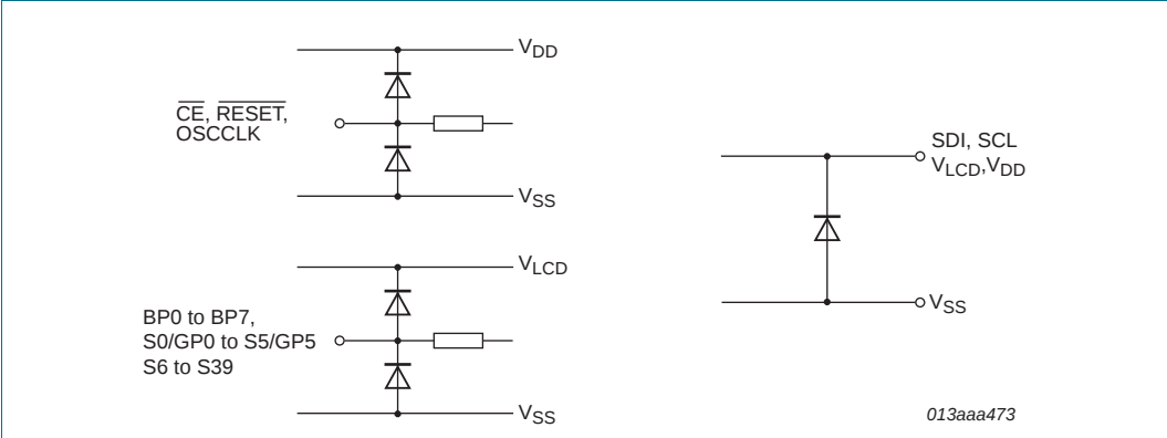
Fig 42. Device protection diagram for PCA8536BT
