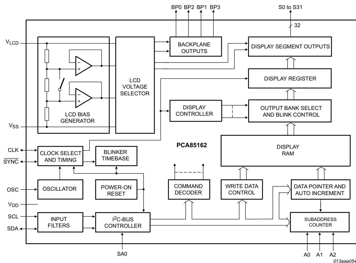
Fig 1. Block diagram of PCA85162
