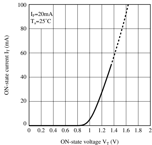
Fig.10 ON-state Current vs. ON-state Voltage
