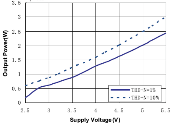
Output Power VS. Supply Voltage R_L=4\Omega
