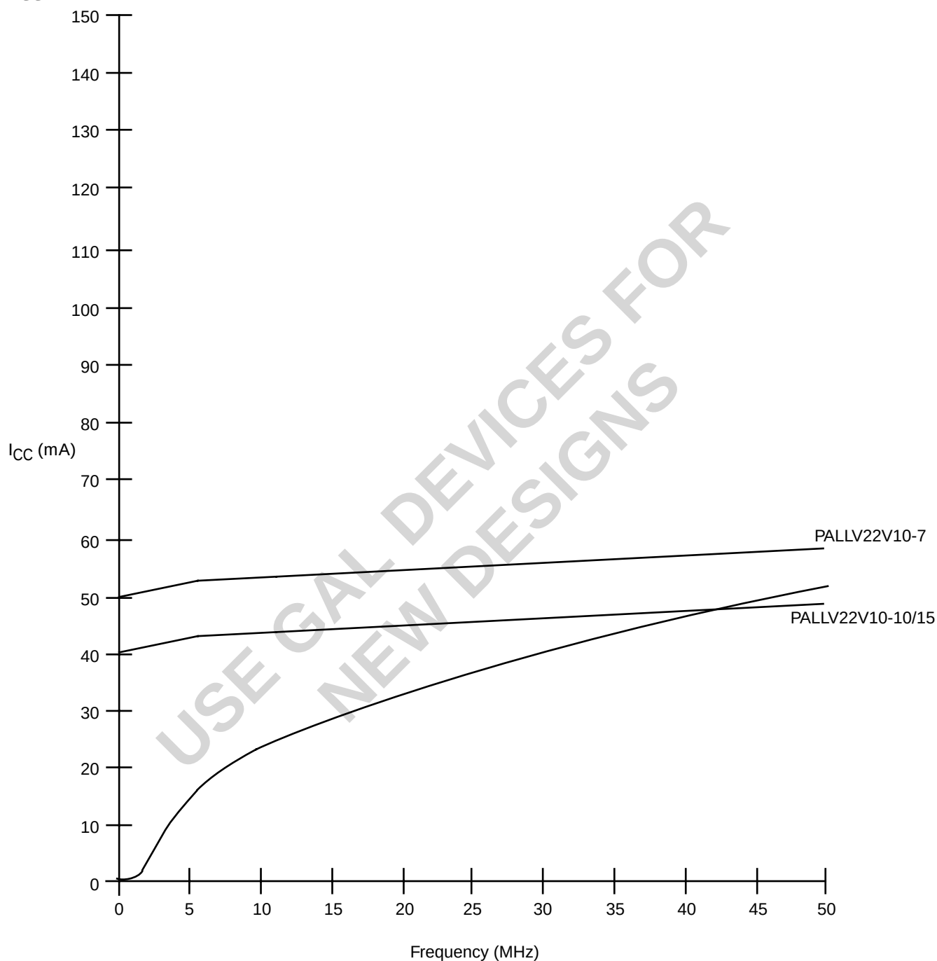
I_{CC} vs. Frequency
