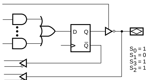
Output Registered/Active Low
