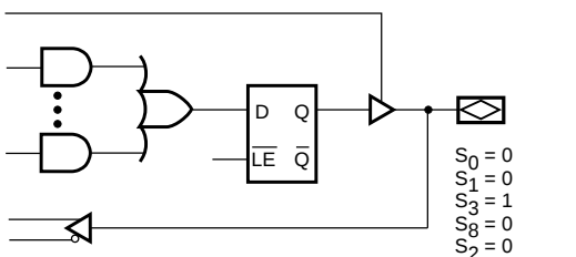
Output Latched/Active High, I/O Feedback
