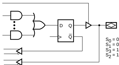
Output Registered/Active High
