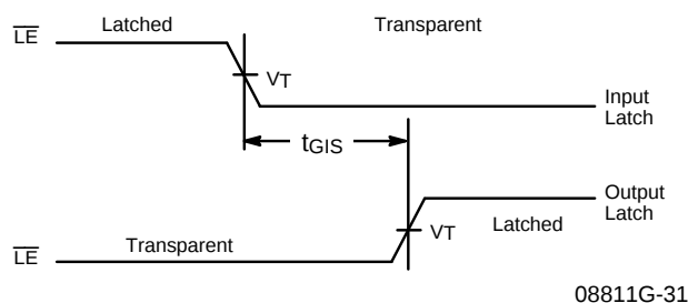
Input and Output Latch Relationship
