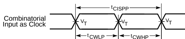
PT Clock Width
