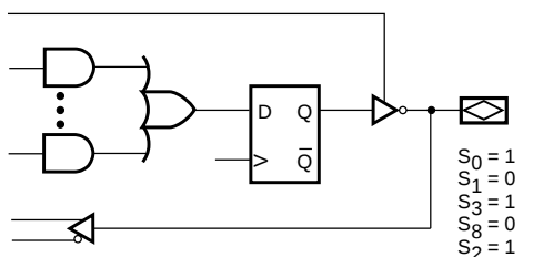
Output Registered/Active Low, I/O Feedback
