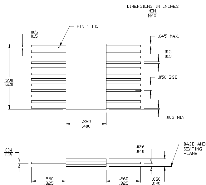
24-Lead Rectangular Cerpack K73 MIL-STD-1835 F-6 Config.A
