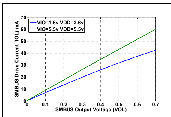
FIGURE 2-18: I^2\text{C}/\text{SMBus} Drive Current vs. V_{OL} .
