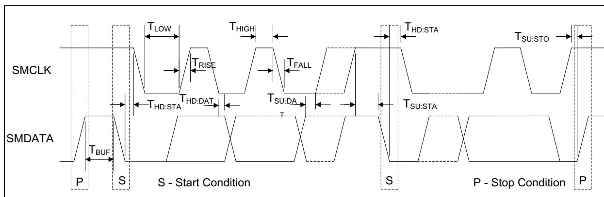
FIGURE 1-1: SMBus Timing.
