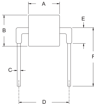
90VAC RADIAL LEAD PACKAGE OUTLINE
