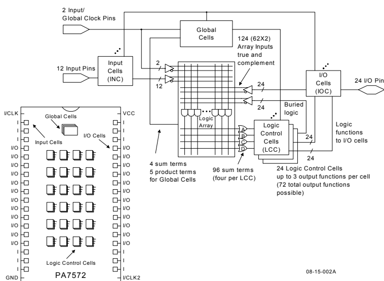
Figure 2. Block Diagram
