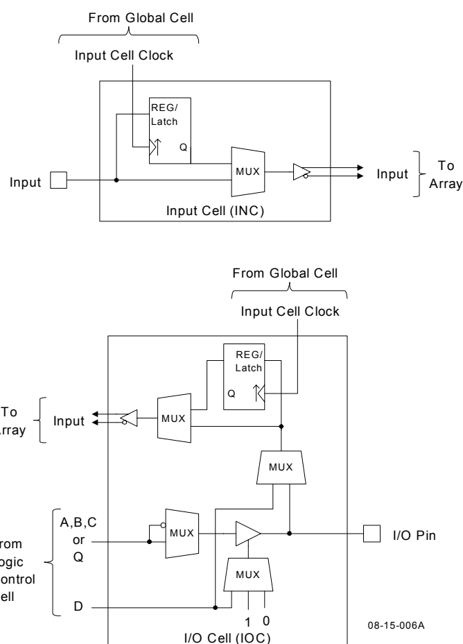
Figure 6. Input and I/O Cell Block Diagrams
