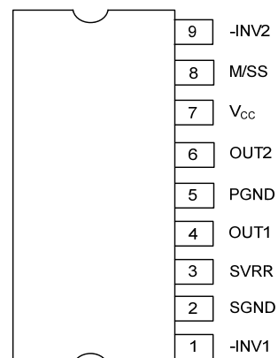
HSIP-9B
