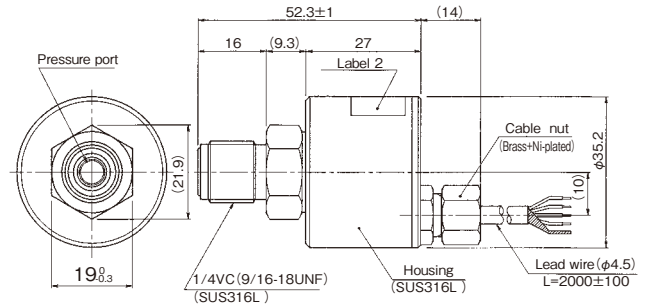
(4) PA-850/PS85, VC type
