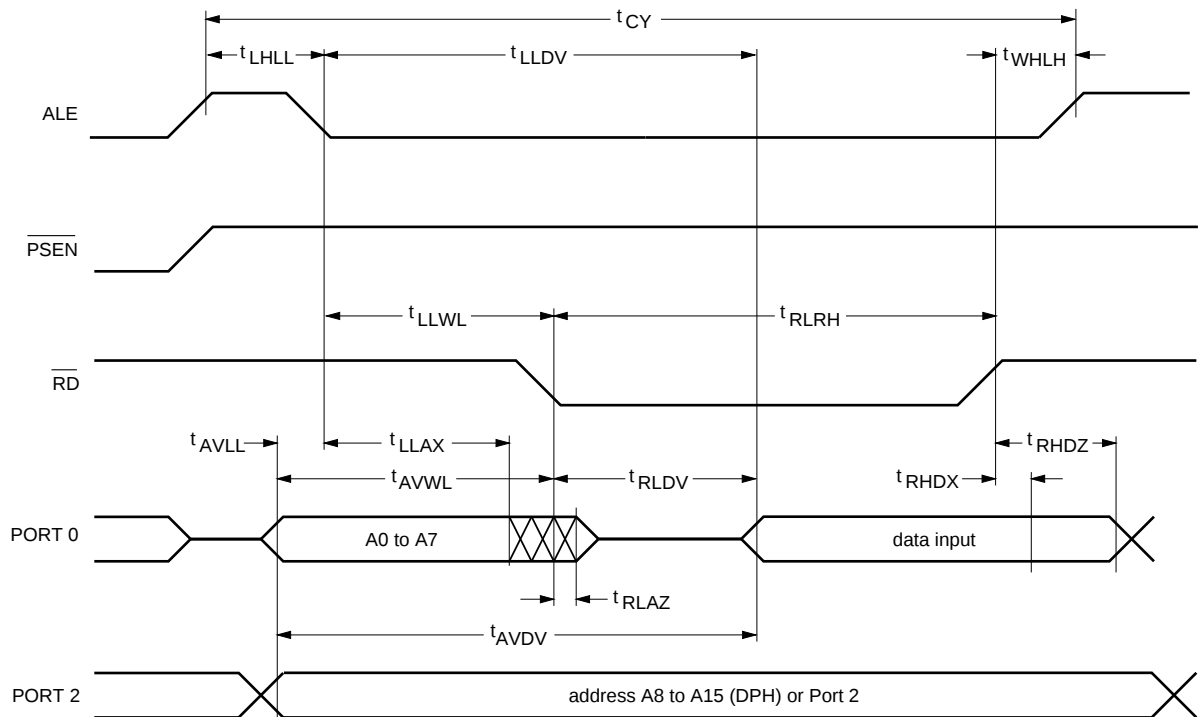
Fig.32 Read from external Data Memory.
