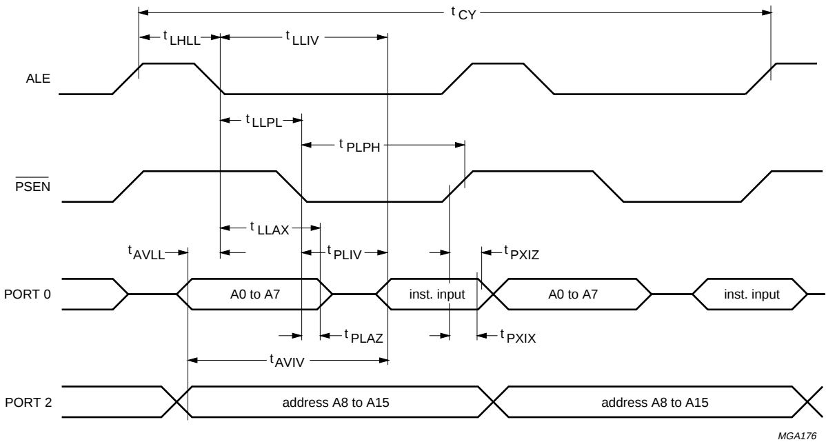
Fig.31 Read from external Program Memory.
