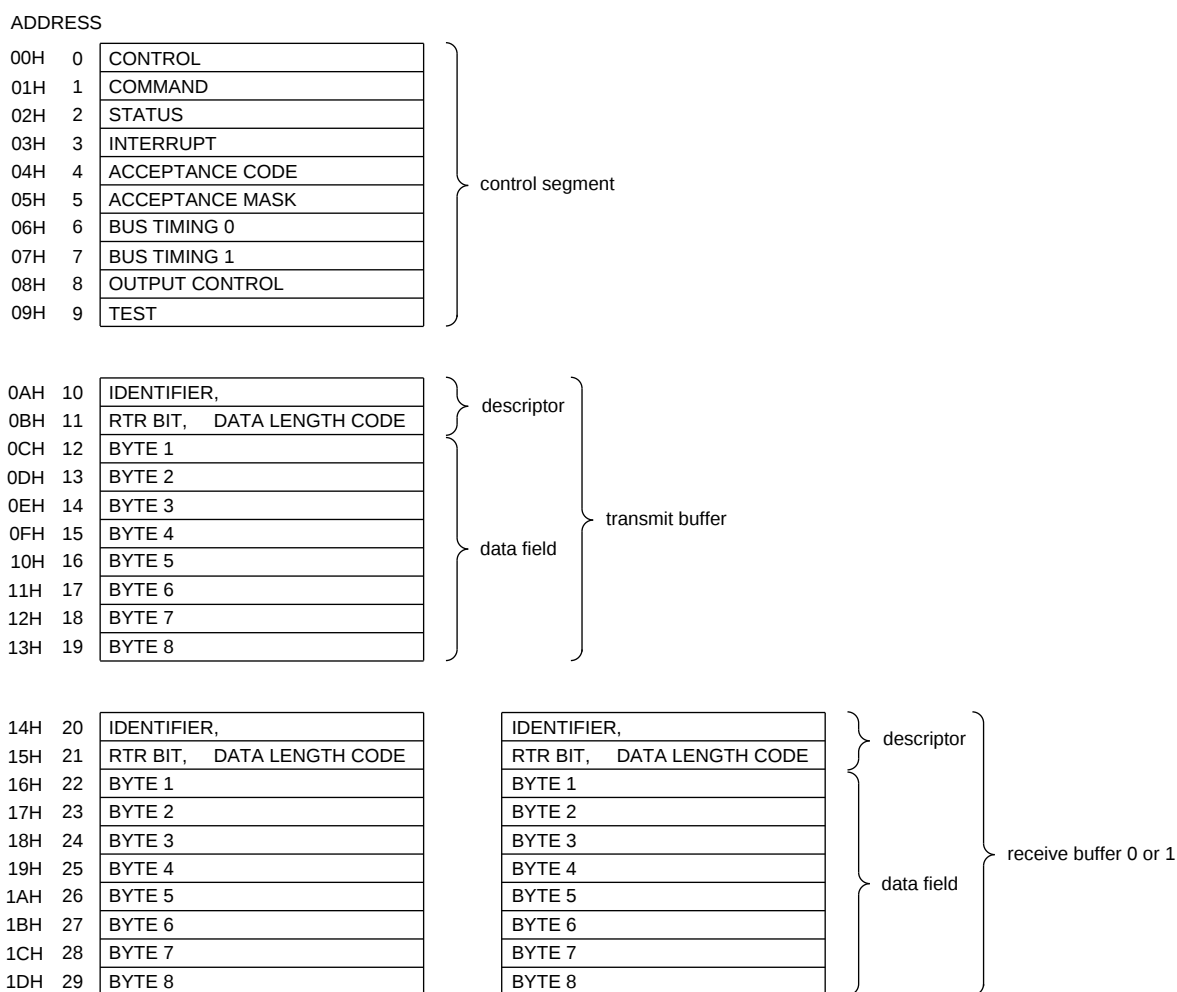
Fig.15 CAN-controller internal address allocation.
