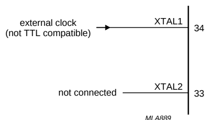
Fig.24 Driving P8xC592 from an external source.
