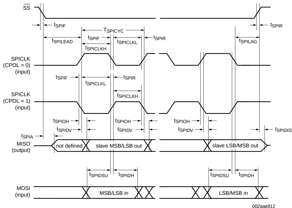
Fig 45. SPI slave timing (CPHA = 1)
