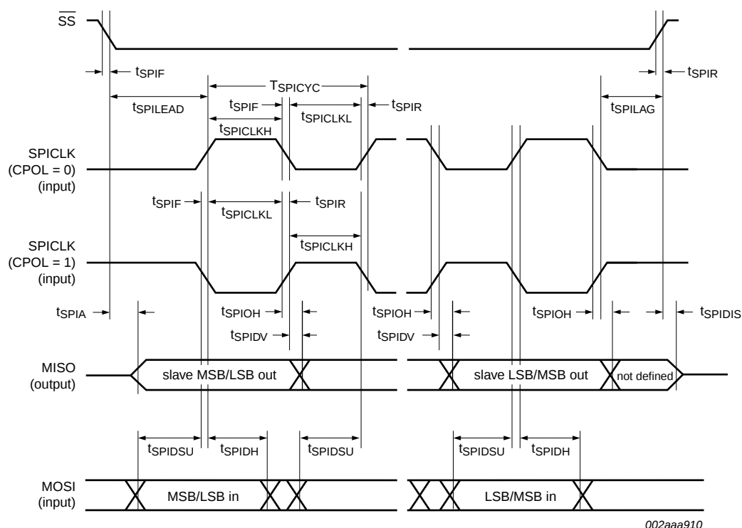
Fig 44. SPI slave timing (CPHA = 0)
