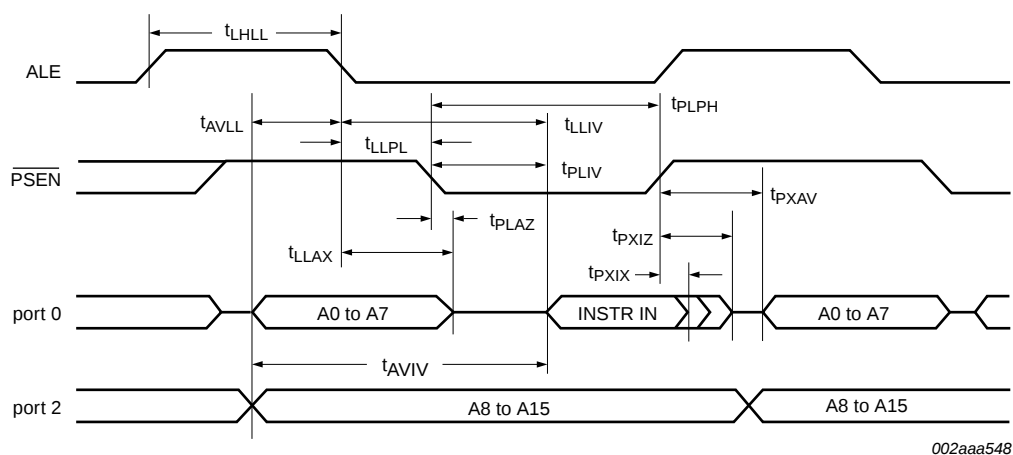
Fig 36. External program memory read cycle
