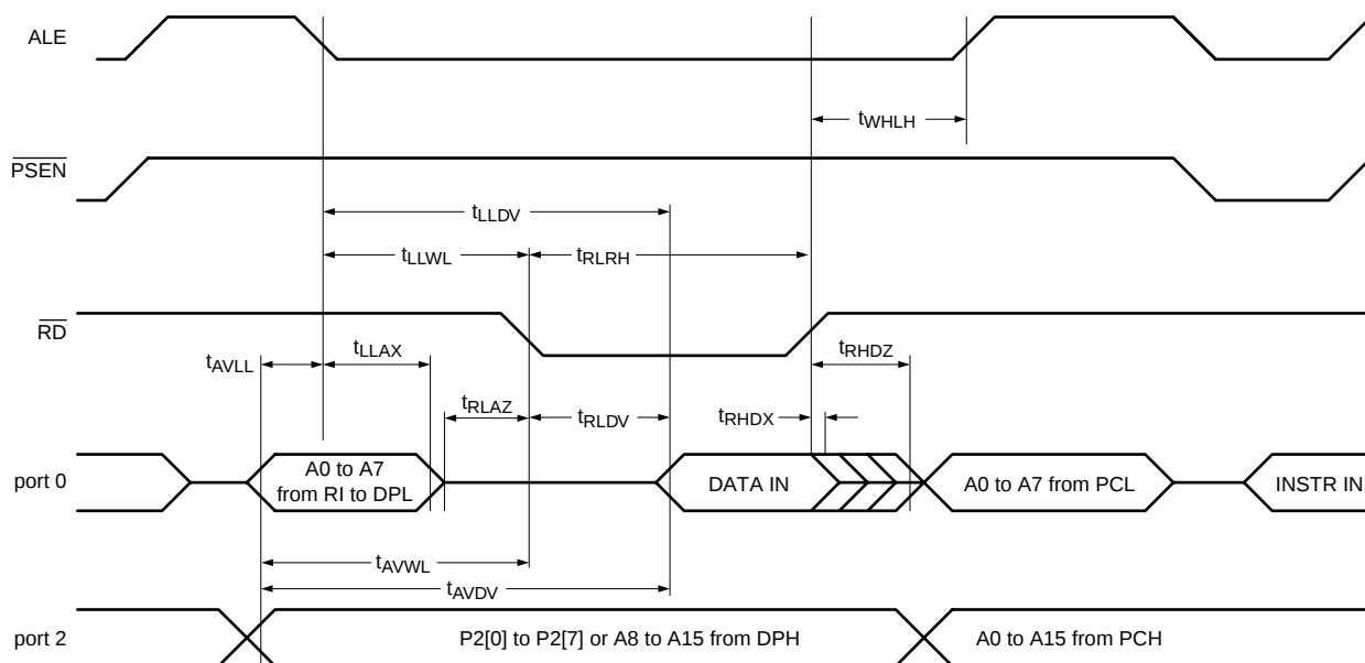
Fig 22. External data memory read cycle
