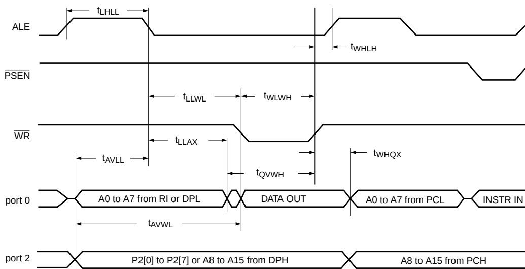
Fig 23. External data memory write cycle
