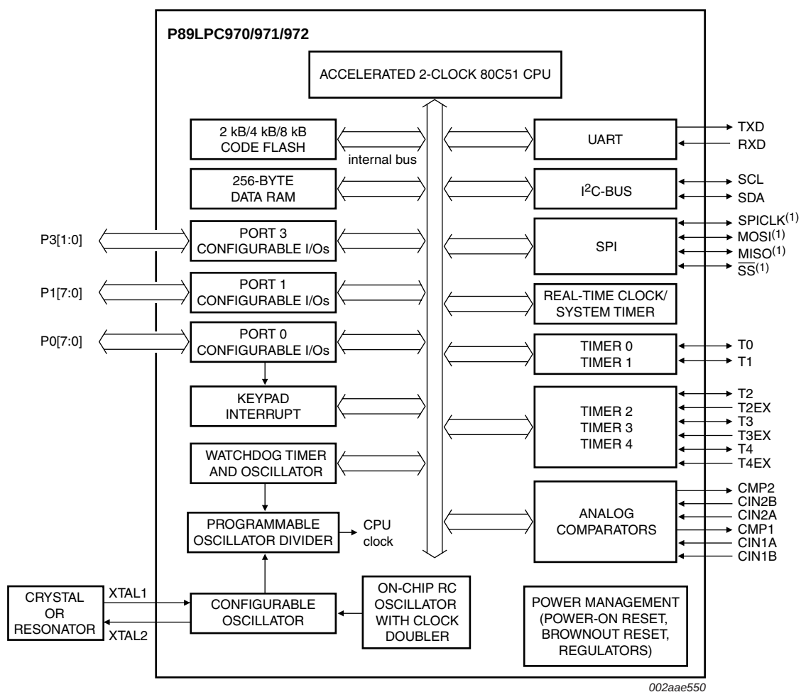
Fig 1. Block diagram
