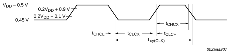
Fig 18. External clock timing
