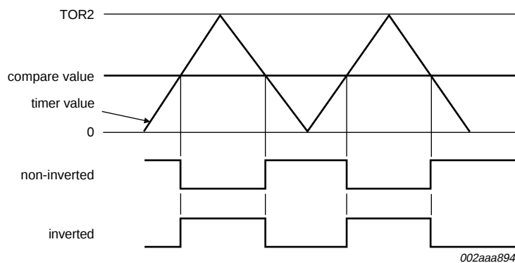
Fig 10. Symmetrical PWM
