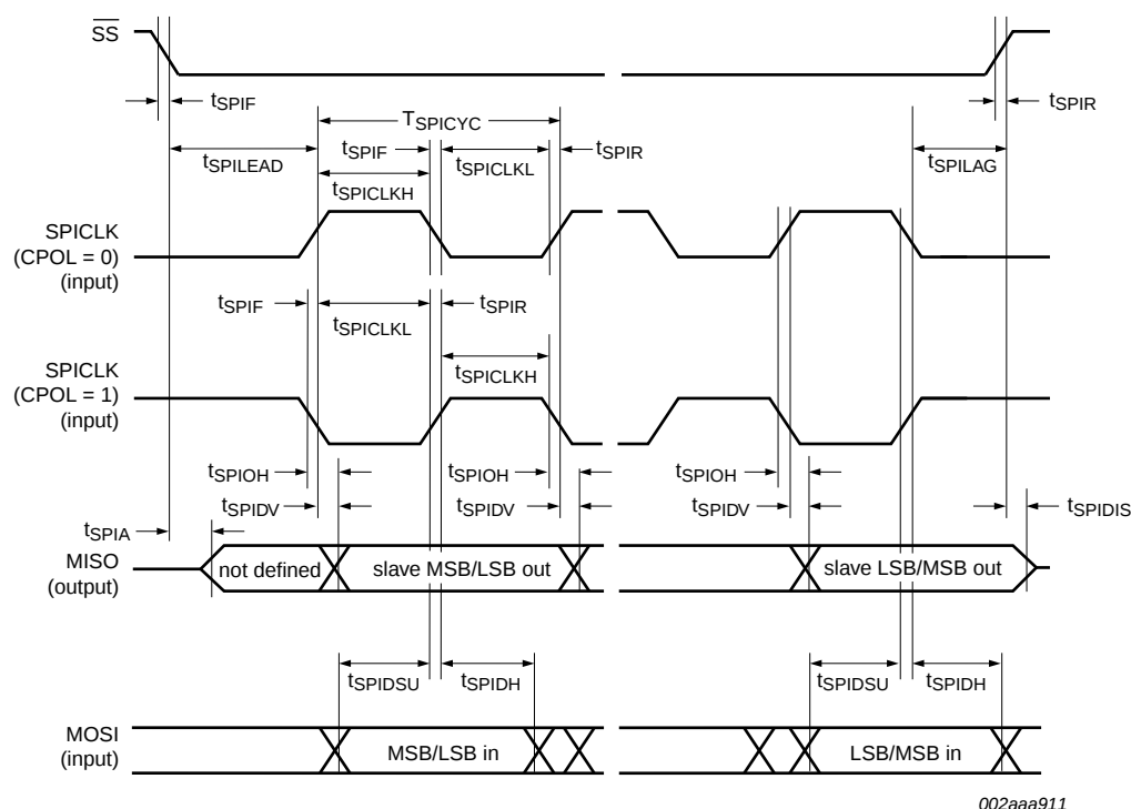
Fig 36. SPI slave timing (CPHA = 1)
