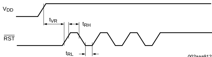
Fig 37. ISP entry waveform
