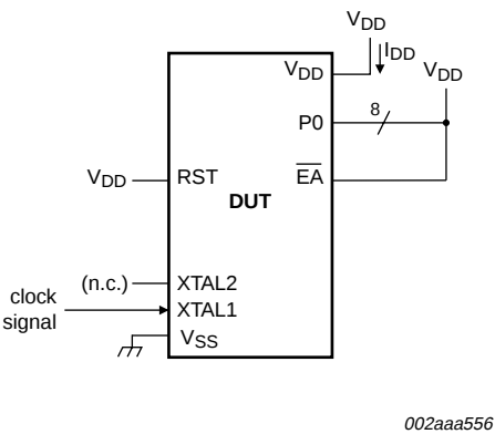
Fig 39. I DD test condition, Active mode
