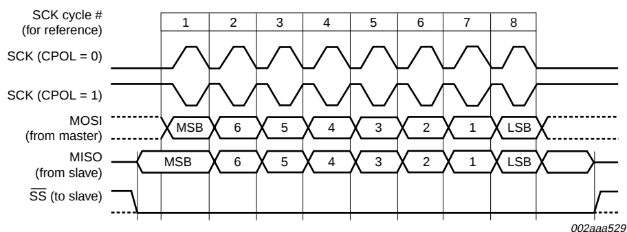
Fig 17. SPI transfer format with CPHA = 0
