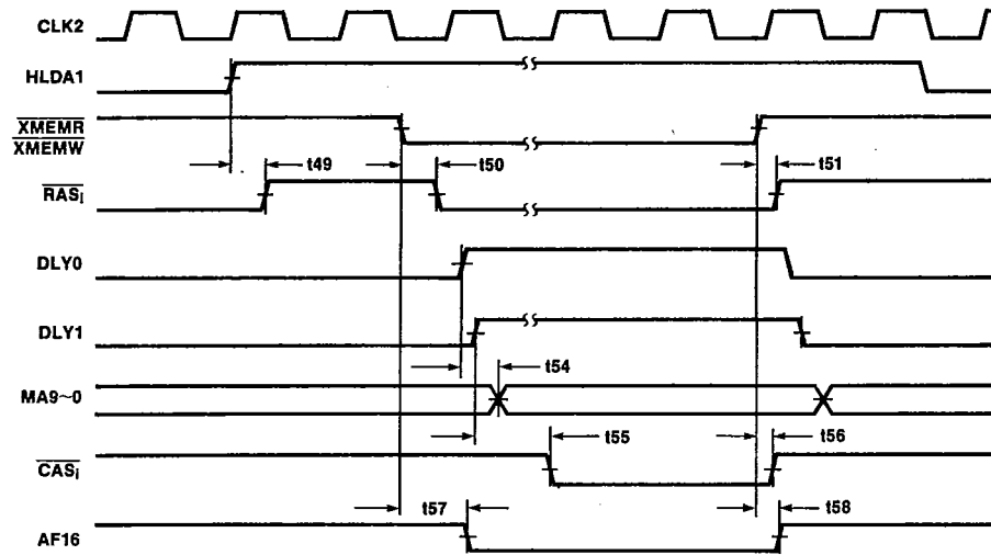
DMA Cycle
