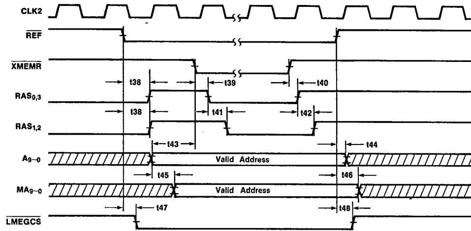
Refresh Cycle
