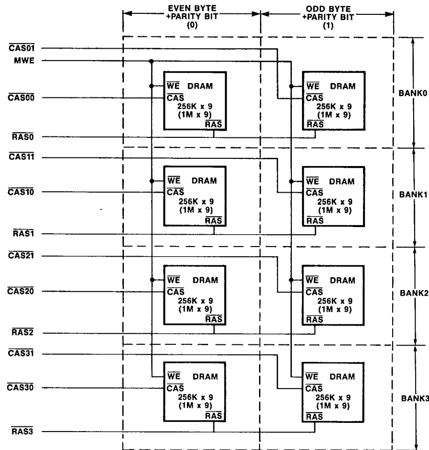
Figure 2.5 DRAM Organization
