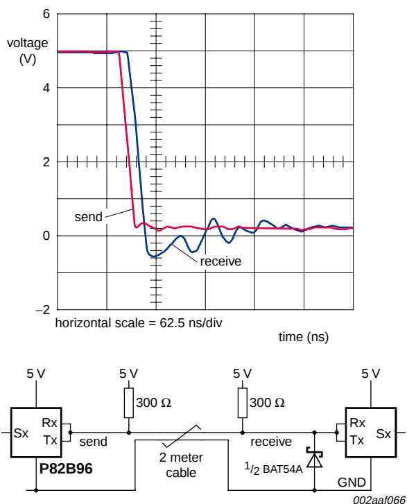
Fig 24. Wiring transients limited by a Schottky diode
