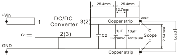
Effeciency and Output Voltage Ripple Test
