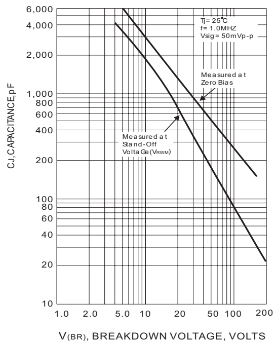
Fig.4 TYPICAL CAPACITANCE
