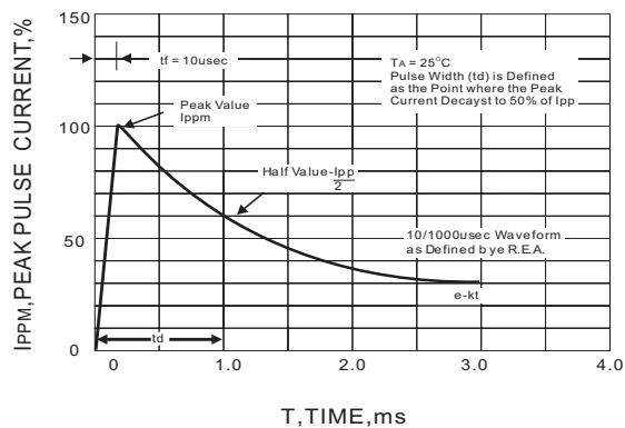
Fig.3 PULSE WAVEFORM
