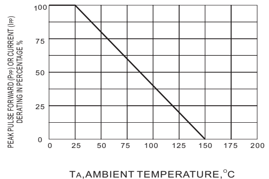
Fig.2 DERATING CURVE
