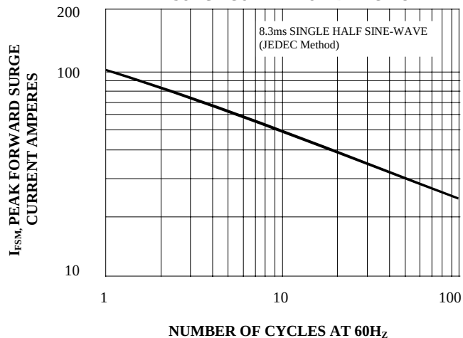
FIG. 7 - MAXIMUM NON-REPETITIVE FORWARD SURGE CURRENT UNIDIRECTIONAL
