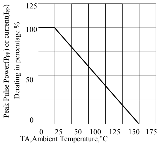
Fig. 2-Pulse Derating Curve
