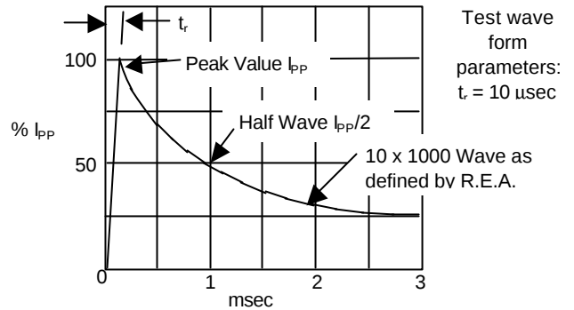
Figure 2 - Pulse Waveform
