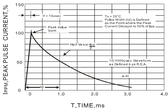
Fig.3 PULSE WAVEFORM
