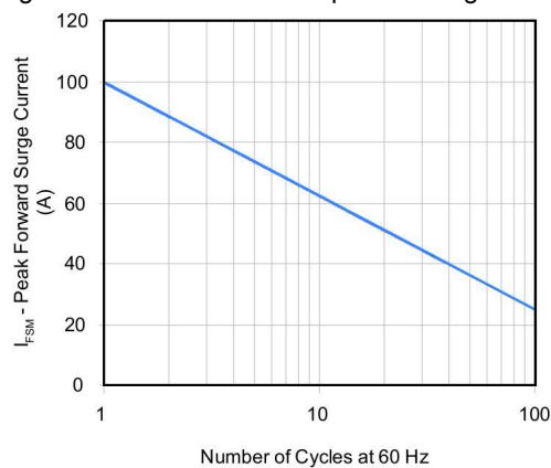
Figure 6 - Maximum Non-Repetitive Surge Current
