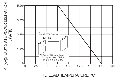
Fig.6 STEADY STATE POWER DERATING CURVE
