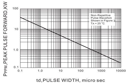
Fig.1 PEAK PULSE POWER RATING PULSE TIME CURVE
